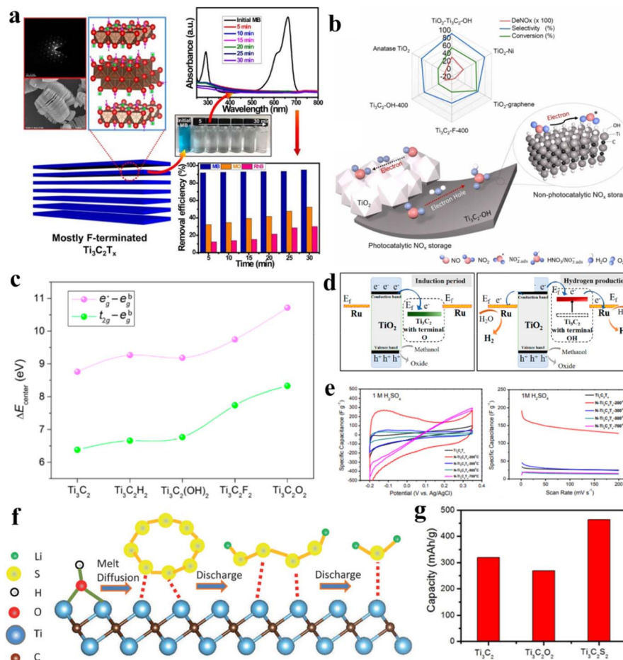
Fig. 10 (a) F-terminated \text{Ti}_3\text{C}_2\text{Tx} MXene used for the removal of methylene blue, reproduced from ref. 358 with permission from Elsevier, copyright 2021. (b) OH-terminated MXene used for photocatalytic reactions, reproduced from ref. 160 with permission from Elsevier, copyright 2022. (c) Energy differences between \text{Ti}_2 3d orbitals in unterminated and terminated MXenes along with their stability order, reproduced from ref. 162 with permission from American Chemical Society, copyright 2017. (d) Charge exchange during photoreactions, reproduced from ref. 169 with permission from American Chemical Society, copyright 2020. (e) Comparative CV results obtained at a scan rate of 1 \text{ mV s}^{-1} , reproduced from ref. 189 with permission from Elsevier copyright 2017. (f) Heat-treatment interaction with polysulfides, reproduced from ref. 188 with permission from Wiley, copyright 2015. (g) Maximum carrying capacities of \text{Ti}_3\text{C}_2 , \text{Ti}_3\text{C}_2\text{O}_2 , and \text{Ti}_3\text{C}_2\text{S}_2 , reproduced from ref. 173 with permission from Royal Society of Chemistry, copyright 2018.
