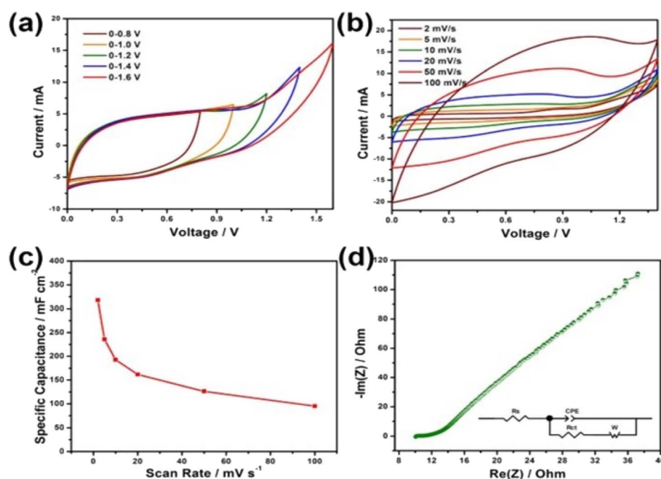
Fig. 25 (a) CV curves of the device at various voltage windows at a sweep rate 20 \text{ mV s}^{-1} ; (b) CV curves; (c) specific capacitance at various sweep rates; and (d) EIS spectrum. Reproduced with permission from ref. 61 Copyright (2017), the American Chemical Society.
