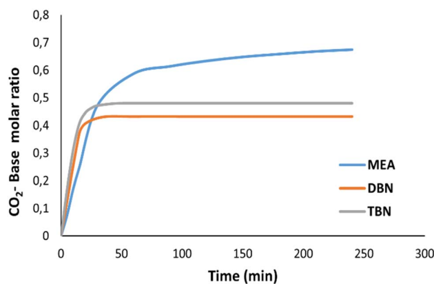
Fig. 4 Absorption time of DBN, TBN and MEA in their respective solvents. Reaction conditions: TBN (30% wt) in butyl acetate, DBN (30% wt) in acetonitrile and MEA (30% wt) in water, at room temperature.
