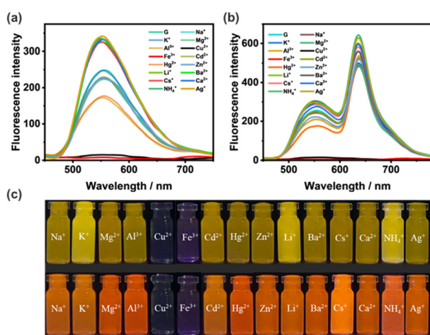
Fig. 4 (a) Fluorescence spectra of G NPs ( 5.00 \times 10^{-5} M, f_w = 90\% ) interacting with different metal ions. (b) Fluorescence spectra of G-NDI NPs ( [\text{G}] = 5.00 \times 10^{-5} M, G/NDI = 200/1, f_w = 90\% ) interacting with different metal ions. [\text{M}^{n+}] = 5.00 \times 10^{-5} M, \lambda_{\text{ex}} = 325 nm. (c) Photograph of compound G (upper) and G-NDI (down) interacting with metal ions under a 365 nm UV lamp.
