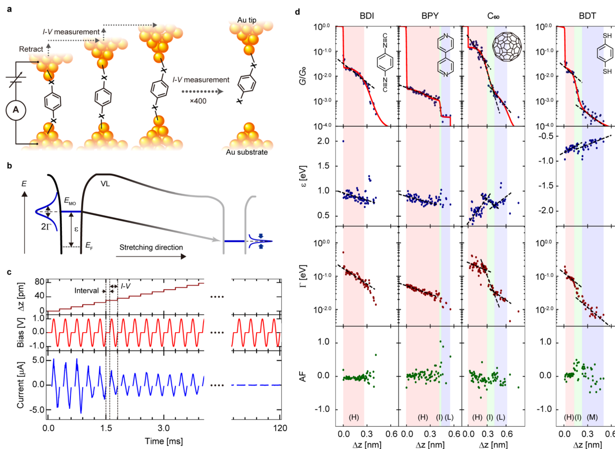
Fig. 1 (a) Schematic illustration showing one cycle of repeated current–voltage ( I–V ) curve measurement during the junction stretching process. (b) Shift of molecular orbital level ( \varepsilon ) and electronic coupling ( \Gamma ) during molecule junction stretching. (c) Time course of \Delta z , bias voltage applied to the junction, and measured current in the magnified time region, in which a molecular junction forms. Here, the zero point of \Delta z is redefined as the display starting point. (d) Conductance ( G ), \varepsilon , \Gamma and asymmetric factor (AF) with junction elongation for BDI, BPY, BDT, and C 60 . The \varepsilon , \Gamma , and AF values are obtained by analyzing I–V curves measured during the junction stretching process in (c). See main text for details. Blue, blue, red, and green dots indicate G , \varepsilon , \Gamma , and AF, respectively. The labels of (H) and (L) indicate the high and low conductance states, and (I) indicates intermediate states between H (M) and L states. The regions of the H, T and L (M) states are filled in red, green, and blue, respectively. See ESI Section 3† for the method used to determine the region of each state. The dotted lines represent the results of a linear fit of the experimental data for each region.
