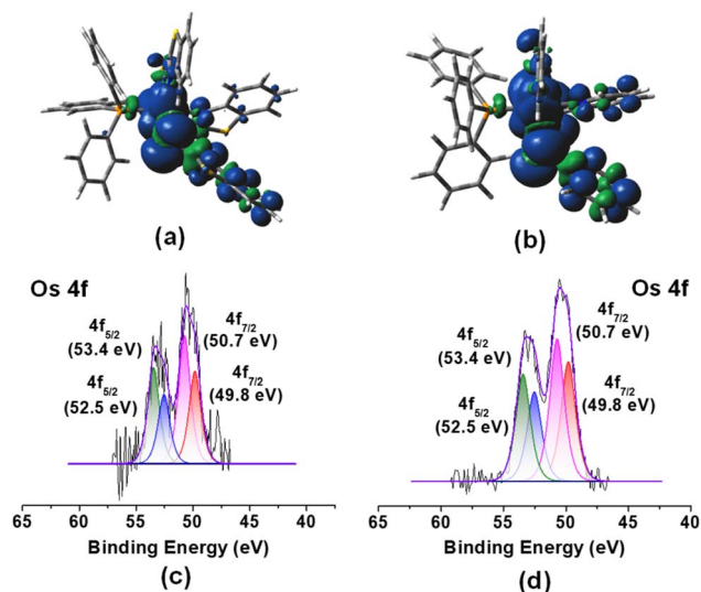
Fig. 2 Spin density plot for 3a (a) and 3b (b) (isovalue 0.004 [ e bohr ^{-3/2} ]); X-ray photoelectron spectroscopy (XPS) spectra of Os 4f_{7/2} and 4f_{5/2} for 3a (c) and 3b (d).
