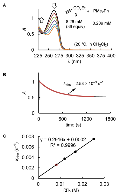
Fig. 2 (A) The decay of the UV absorption of \text{PMe}_2\text{Ph} was used to monitor the kinetics of the reaction of \text{PMe}_2\text{Ph} with ethyl propiolate (3) in \text{CH}_2\text{Cl}_2 under pseudo first-order conditions (proton source: CT, [\text{CT}]_0 = 0.232 \text{ mM} ). (B) Exponential decay of the absorption A at 252 nm during the reaction. (C) Determination of the second-order rate constant k_2 \text{ (M}^{-1} \text{ s}^{-1}\text{)} from the slope of a linear correlation of k_{\text{obs}} \text{ (s}^{-1}\text{)} vs. [\text{3}]_0 .
