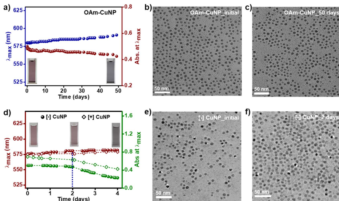
Fig. 3 Colloidal stability studies of OAm, [−], and [+] CuNPs. Time-dependent monitoring of UV-vis absorption of (a) OAm-CuNPs in toluene, (d) [−] and [+] CuNPs in water. Representative large-area TEM images of the corresponding CuNPs taken (b), (e) immediately after the synthesis and (c), (f) after a few days, as mentioned in the image. Negligible changes in the time-dependent absorption and TEM studies confirm the excellent colloidal stability of OAm-CuNPs in toluene for at least 50 days under ambient conditions. On the other hand, [−] CuNPs and [+] CuNPs could only retain their stability in aqueous medium for ~2 days under inert conditions. This lower stability could be attributed to the faster oxidation of CuNPs in water, compared to toluene.
