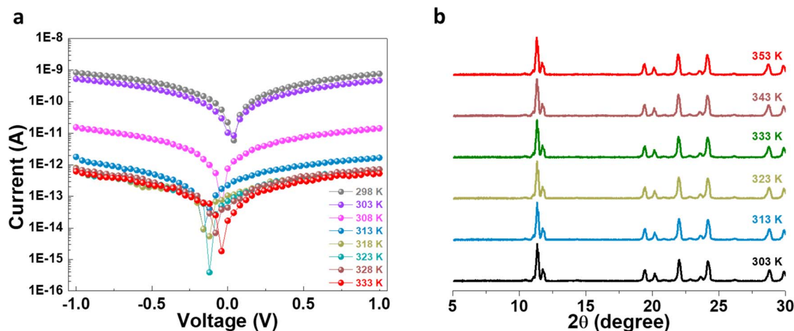
Fig. 4 Metallic conduction without structural change. (a) Variable-temperature current–voltage ( I – V ) diagram of (TMA)AgBr 2 in the temperature range from 298 K to 333 K, illustrating thermally deactivated charge transport. (b) Variable temperature PXRD patterns showing the retention of the structural phase over the temperature range.
