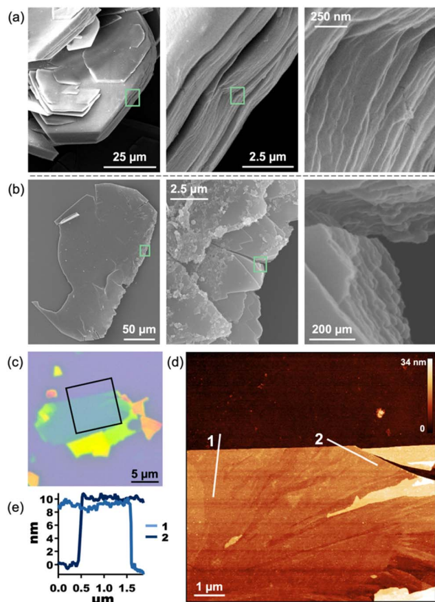
Fig. 4 SEM of MOFs 1 (a) and 2 (b) with progressively magnified images (left to right) showing the layers of the crystals' edges. Optical image (c) of an exfoliated flake of 2 on a Si/SiO 2 wafer, its AFM topography map (d), and height profile (e).
