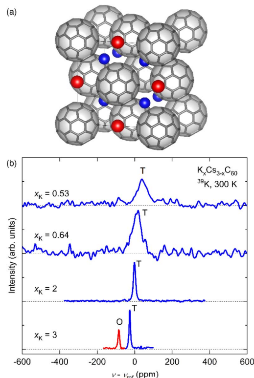
Fig. 1 (a) Crystal structure of fcc fullerides (space group Fm\bar{3}m ) with stoichiometry A_3C_{60} (A is an alkali metal cation; blue spheres depict cations residing in tetrahedral (T) and red in octahedral (O) interstices, respectively). The \text{C}_{60}^{3-} units are merohedrally disordered; here only one of the two possible orientations is depicted at each lattice position. (b) ^{39}\text{K} NMR spectra measured for K_xCs_{3-x}C_{60} (refined x_K = 0.53, 0.64, 2, 3 ) powders at 300 K. The T and O peaks are labelled in blue and red colour, respectively. The spectrum of K_{3-x}Cs_xC_{60} ( x = 3 ) is being reproduced from ref. 24.
