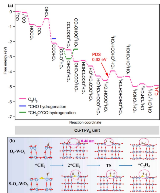
Fig. 2 (a) Gibbs free energy diagrams of CO 2 reduction on the Cu–Ti–V 2 O unit. This figure has been reproduced from ref. 46 with permission from Springer Nature, copyright 2023. (b) The C–C coupling process of Ov–WO 3 and S–Ov–WO 3 . This figure has been reproduced from ref. 47 with permission from Elsevier, copyright 2023.
