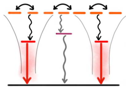
Fig. 4 Schematic state diagram of a doped NP system with indication of energy migration between multiple similar (donor) dyes in the NP. Efficient energy transfer to a low number of isolated dopant (acceptor) dyes outcompetes quenching by the trap state.
