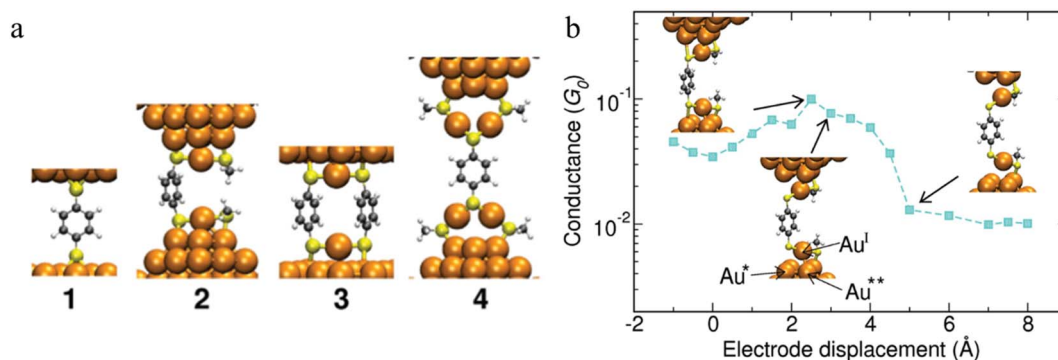
Fig. 17 (a) Structures of the junctions 1–4 at mechanical equilibrium; (b) conductance of junction 2 vs. the electrode displacement. The insets (from left to right): maximal strain of the S–Au * bond corresponding to the maximal conductance, breaking of the S–Au * bond, reflected in drop of the conductance, and subsequent elongation and breaking of the Au I –Au ** bond. The conductance stays the same after the Au I –Au ** bond is broken. Further stretching of RS–Au I –BDT–Au I –SR unit does not affect the conductance since the BDT is decoupled from the gold electrodes. Figures adapted with permission from ref. 87. Copyright 2010, American Chemical Society.
