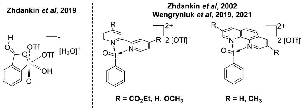
Fig. 5 Recently reported hypervalent I(V) compounds possessing high oxidative capacity.
