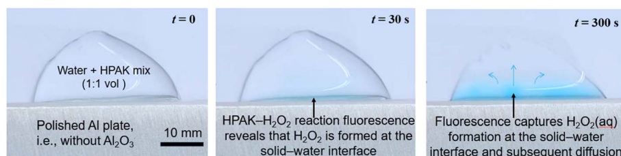
Fig. 3 Time-dependent formation of H 2 O 2 (aq) in a macroscopic droplet of a 1 : 1 mixture of water and HPAK reaction mixture on an Al plate (see ESI Movie S1†). Within seconds, H 2 O 2 (aq) formation at the Al–water interface is evident, proving that the size of the droplet and air–water interface do not matter. The solid–water interface drives this chemical transformation. The Al surface is superhydrophilic, and water spreads on it as a film. Therefore, the Al plate was placed vertically on a polystyrene sheet and formed a 1 ml droplet resting on the Al edge. The 1 : 1 mixture of water and HPAK reaction on polystyrene did not yield the faintest blue fluorescence visible to the naked eye.
