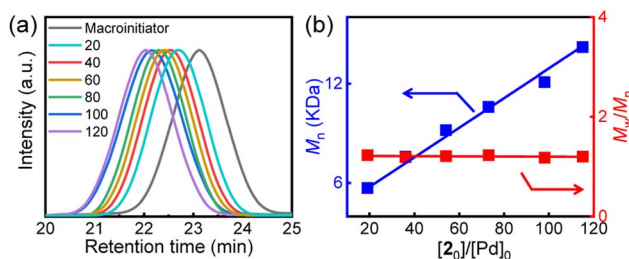
Fig. 1 (a) SEC curves for the copolymerization of 2 initiated by R -poly- 1 105 carrying the Pd(II)-terminus at different 2 -to-Pd(II) ratios. (b) Plots of M n and M w / M n of R -poly( 1 m - b - 2 n )s vs. the 2 -to-Pd(II) ratios.
