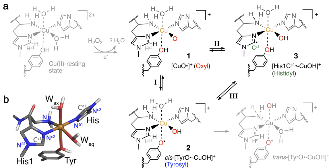
Fig. 1 (a) Formation of Cu(II)-oxyl 1 from the Cu(II)-resting state (in gray) with a reductant and \text{H}_2\text{O}_2 , and generation of intermediates 2 and 3 from 1 . Intermediates 1 – 3 (in black) are investigated here for their role as part of oxidative damage or protective pathways (species in gray are not included in this study). (b) Ball-and-stick model of the first coordination sphere of the QM/MM optimized Cu(II)-resting state of LsAA9 employing TPSS/def2-SV(P).
