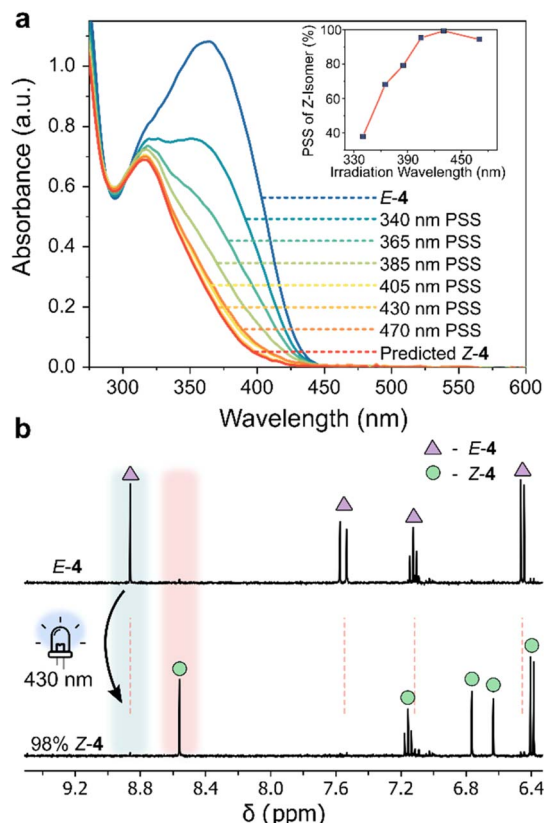
Fig. 3 (a) UV/vis absorption spectra of 4 (170 \mu M, 20 °C, MeCN) at various photostationary states (PSS), and the spectrum of the Z -isomer obtained as described in Section 4.5 of the ESI† 59 (inset) Z -isomer percentage generated at different irradiation wavelengths (Table S4†). (b) 1 H NMR spectra (400 MHz, 298 K, CD 3 CN) of E - 4 (triangle), highlighting the emergence of new signals attributed to Z - 4 (circle) upon 430 nm photoirradiation.
