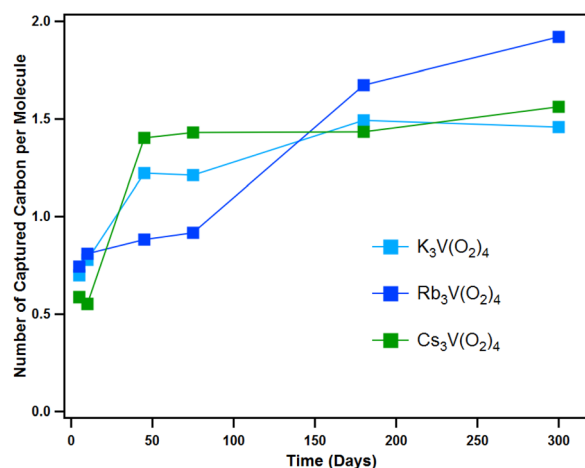
Fig. 8 Carbon capture performance for the three \text{A}_3\text{V}(\text{O}_2)_4 analogues under ambient conditions evaluated by CHN analysis.
