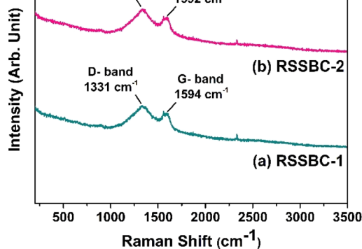
Fig. 6 Raman spectra of (a) RSSBC-1 and (b) RSSBC-2 biochar samples, prepared from rubber seed shell biomass.
