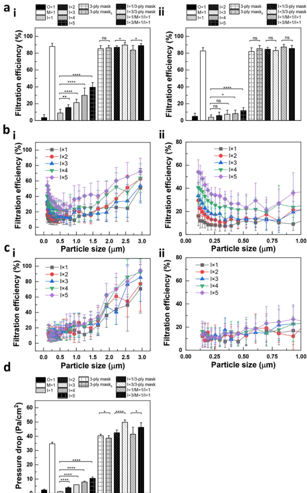
Fig. 1 Filter performance of bare fabrics. Filtration efficiency and breathability were performed according to NIOSH 42CFR84 and ASTM F2100-19e1 standards, respectively. (a) Overall filtration efficiency of bare fabrics tested with 5% NaCl aerosol (i) and DOP aerosol (ii). ( n = 10-21 for a(i) and 13-24 for a(ii), mean \pm SD). (b and c) Particle size-dependent filtration efficiency tested with 5% NaCl aerosols (b) and DOP aerosols (c) (i: filtration efficiency of bare fabrics and ii: zoomed-in filtration efficiency of the bare fabrics). ( n = 7-21 for b and 9-24 for c, mean \pm SD). (d) Breathability of bare fabrics with different stacking sequences ( n = 9-12 , mean \pm SD). For all panels: ns, P > 0.05 ; *, P < 0.05 ; **, P < 0.01 and ****, P < 0.0001 by one-way ANOVA. The obtained fabrics were labelled as Fabric Salt \times #Amount. 'Fabric' indicates PP fabric type (I, M, O); 'Salt' the coating (T20, NaCl, KCl, K 2 SO 4 ); '#' the number of layers (1-5); 'Amount' the coating weight (5, 9, 13 mg cm -2 ). Bare fabrics are "Fabric \times #", '#' being the layer count. The '/' symbol shows layer order, 'A/B' means A over B.
