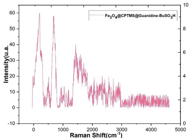
Fig. 7 Raman spectra of \text{Fe}_3\text{O}_4\text{@CPTMS@guanidine-BuSO}_3\text{H} MNPs.
