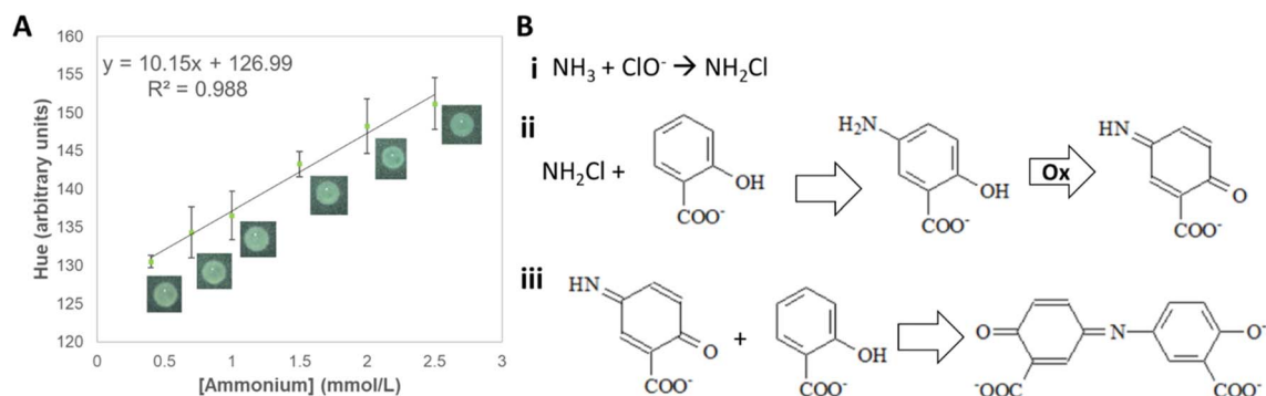
Fig. 5 Detection of ammonium in the proposed \mu\text{PAD} . (A) Calibration curve obtained for ammonium in concentrations ranging from 0.5 to 2.5 \text{mmol L}^{-1} . (B) Reaction between (i) ammonium and hypochlorite, forming monochloramine; (ii) monochloramine and salicylate, forming 5-aminosalicylate and (iii) 5-aminosalicylate being oxidized in the presence of nitroprusside catalyst forming the blue colored indosalicylate compound.
