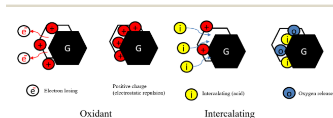
Fig. 7 The mechanism scheme of graphite expansion of HETG.
