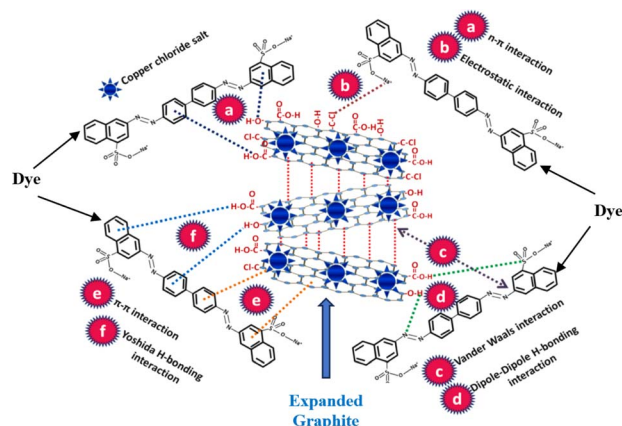
Fig. 15 Potential interactions that contribute to the process of dye adsorption on the EG. Reprinted with permission from ref. 93.
