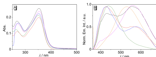
Fig. 1 Absorption ( c = 10 \mu\text{M} ) (A) and normalized emission spectra (B) ( \lambda_{\text{ex}} = 350 \text{ nm} ) of 3 in \text{H}_2\text{O} (green), DMSO (blue), MeOH (black), EtOH (magenta), MeCN (red), and glycerol (orange).
