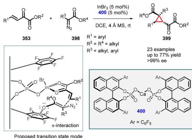
Scheme 89 Binary Lewis acid ( \text{InBr}_3 and chiral calcium phosphate) catalyzed enantioselective MIRC cyclopropanation.
