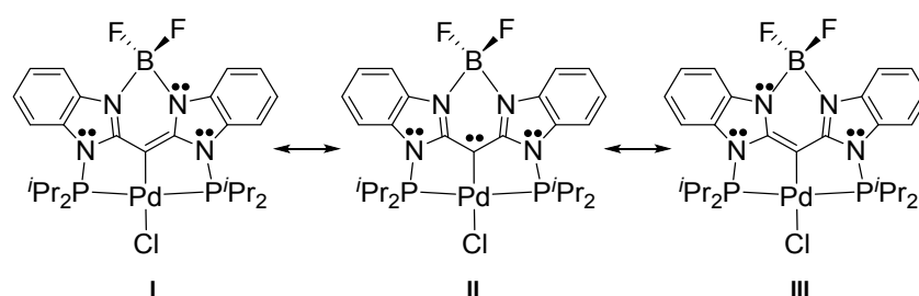
Figure 3. Main resonance structures for 7-Pd .
