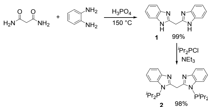
Scheme 1. Synthesis of binucleating ligand 2 .
