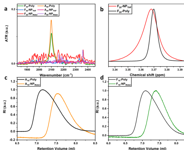
Fig. 1 (a) ATR-IR absorption spectra for F 30 -poly, F 30 -NP THF/water , A 30 -poly and A 30 -NP THF/water . (b) 1 H-NMR spectra in CDCl 3 of F 20 -poly (black) and F 20 -NP THF (red). SEC curves in THF for (c) A 10 -poly and A 10 -NP water and (d) F 10 -poly and F 10 -NP water .
