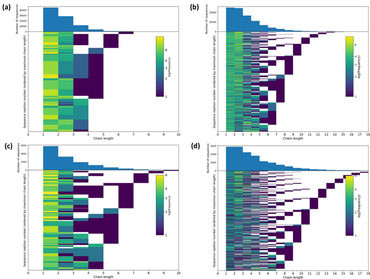
Fig. 6 2D histograms of sequence number against sequence length, with the 1D histogram above, for \text{PLA}_{20} - \text{PCL}_{20} (sample 8 ), where (a) is \epsilon -CL and (b) is L, and for \text{PCL}_{10} - \text{PLA}_{20} - \text{PCL}_{10} (sample 9 ), where (c) is \epsilon -CL and (d) is L.
