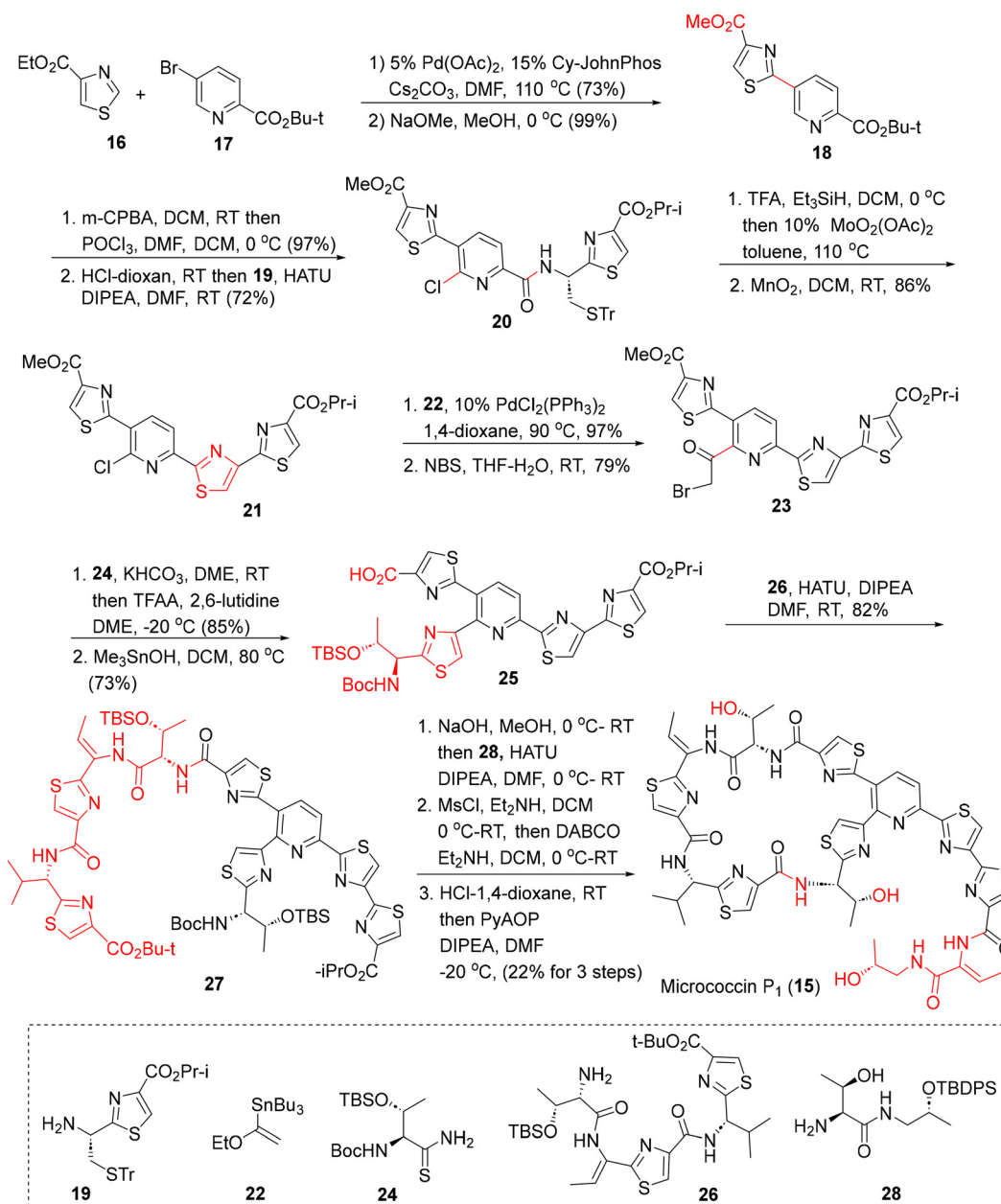
Scheme 1 The Walczak synthesis of micrococcin P 1 ( 15 ). 34a
