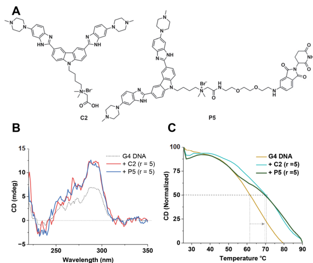
Fig. 4 (A) Chemical structures of molecules C2 and P5. (B) CD spectra of 3 \mu M Hum 21-mer G4 DNA alone, and with compounds C2 and P3 (15 \mu M) in 10 mM Tris-HCl (pH 7.4) containing 0.1 M KCl and 0.1 mM EDTA. (C) CD melting profiles of the pre-formed Hum 21-mer G4 DNA alone, and G-quadruplex DNA incubated with ligands C2 and P5 (15 \mu M) in 10 mM Tris-HCl (pH 7.4) containing 0.1 M KCl and 0.1 mM EDTA.
