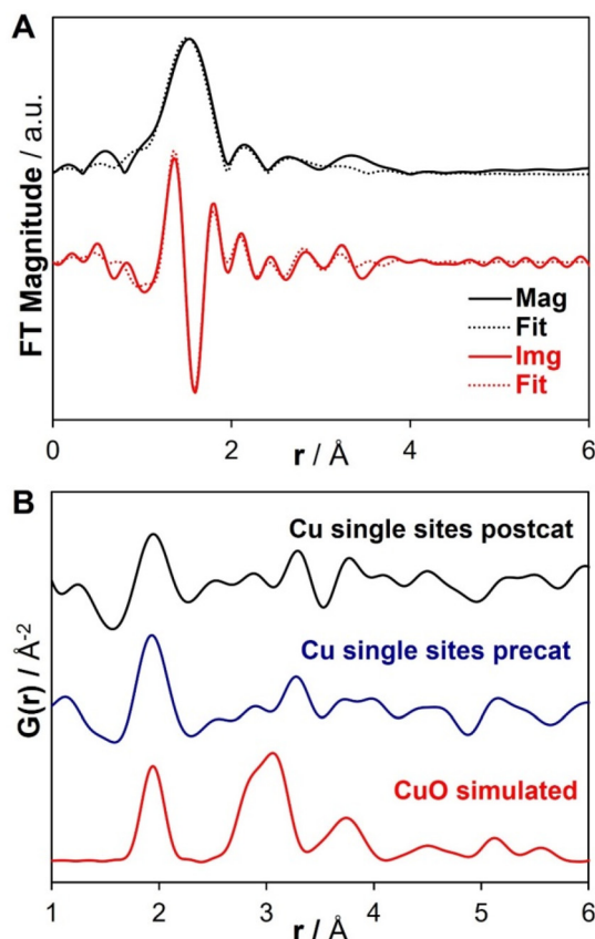
Fig. 7 (A) EXAFS k^2 -weighted Cu K-edge \text{Mag}[χ(r)] and \text{Img}[χ(r)] (solid lines) spectra with their respective fits (dash lines) of Cu-MOF-808@PVDF after catalysis. (B) PDF characterization of the Cu single sites in the MMMs before and after catalysis compared with CuO data.
