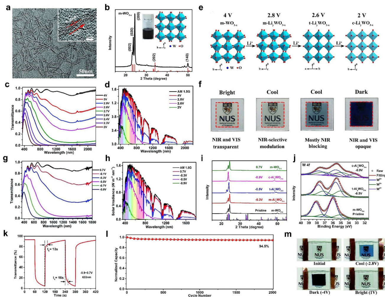
Fig. 7 (a) TEM image, (b) XRD pattern of m-WO 3-x NWs. (c) Optical transmittance spectra, (d) solar irradiance spectra of the m-WO 3-x NW film. (e) Crystal structures and (f) corresponding photos of m-WO 3-x NW films at 4 V, 2.8 V, 2.6 V, and 2 V (vs. Li + /Li), respectively. (a–f) Adapted with permission from ref. 44. Copyright 2018, Royal Society of Chemistry. (g) Transmittance spectra, (h) solar irradiance spectra, (i) XRD patterns, (j) W 4f XPS spectra, (k) switching speed, (l) cycling stability of m-WO 3-x NW films in Al 3+ -based electrolyte. (m) Digital photos of the Al 3+ -based device. (g–m) Adapted with permission from ref. 61. Copyright 2018, Royal Society of Chemistry.
