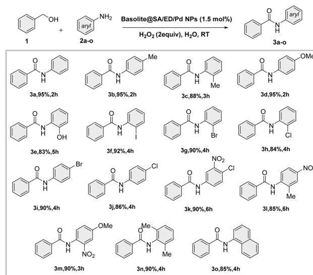
Scheme 3 Tandem oxidative amidation of benzylic alcohol with various anilines.
