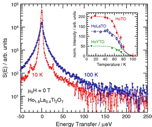
Fig. 11 S(E) of \text{Ho}_{1.6}\text{La}_{0.4}\text{Ti}_2\text{O}_7 at 10 and 100 K in zero field, showing the dominance of the central quasielastic line due to electronic spin flips. The inset shows the temperature dependence of the inelastic excitation for the three Ho samples: \text{Ho}_2\text{Ti}_2\text{O}_7 ( \bullet ), \text{Ho}_{1.6}\text{La}_{0.4}\text{Ti}_2\text{O}_7 ( \square ), and \text{Ho}_{0.7}\text{Y}_{1.3}\text{Ti}_2\text{O}_7 ( \blacktriangledown ). Reprinted with permission from ( Phys. Rev. Lett. , 2009, 102 , 016405). Copyright (2009) American Physical Society.
