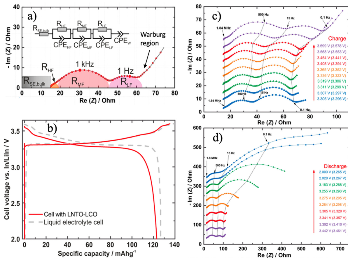
Fig. 4 (a) EIS Nyquist plot with equivalent circuit model simulation to assign a different frequency range to specific resistances; (b) a comparison of LNTO–LCO and liquid electrolyte in the initial galvanostatic charging–discharging profile; SOC dependent Nyquist plot at (c) charging and (d) discharging to highlight the dynamic change of interfacial resistances under different scenarios. Reproduced from ref. 48 with permission from American Chemical Society, copyright 2017.
