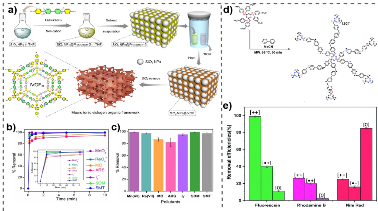
Fig. 2 (a) Synthetic route for iVOF m . (b) and (c) Removal kinetics and % removal of all pollutants through iVOF m . Reproduced with permission from ref. 58. Copyright 2022 Wiley-VCH. (d) Schematic representation of the synthesis of COP 1 + . (e) Bar graphs of adsorption capacities of the cationic, radical-cationic and neutral forms of COP 1 for fluorescein, rhodamine B, and Nile Red. Reproduced with permission from ref. 59. Copyright 2014 the Royal Society of Chemistry.
