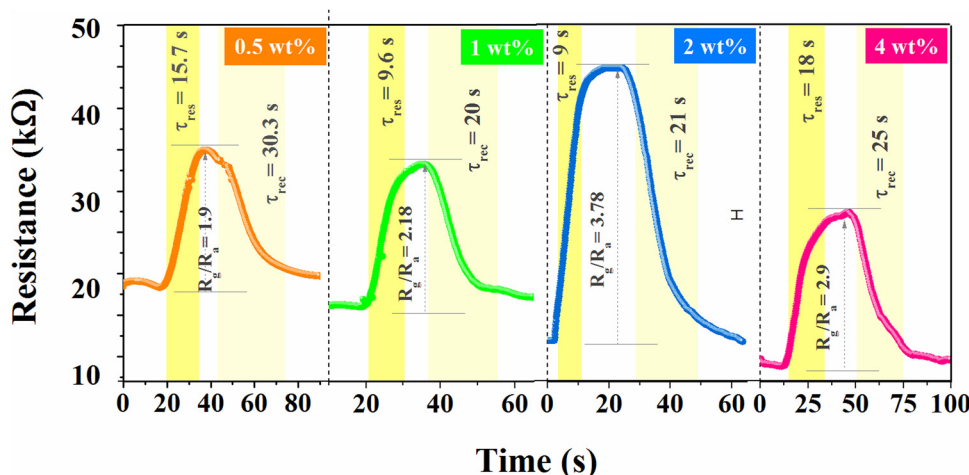
Fig. 8 Effect on \text{NO}_2 sensing behavior with variation in rGO concentration (0.5–4 wt%).
