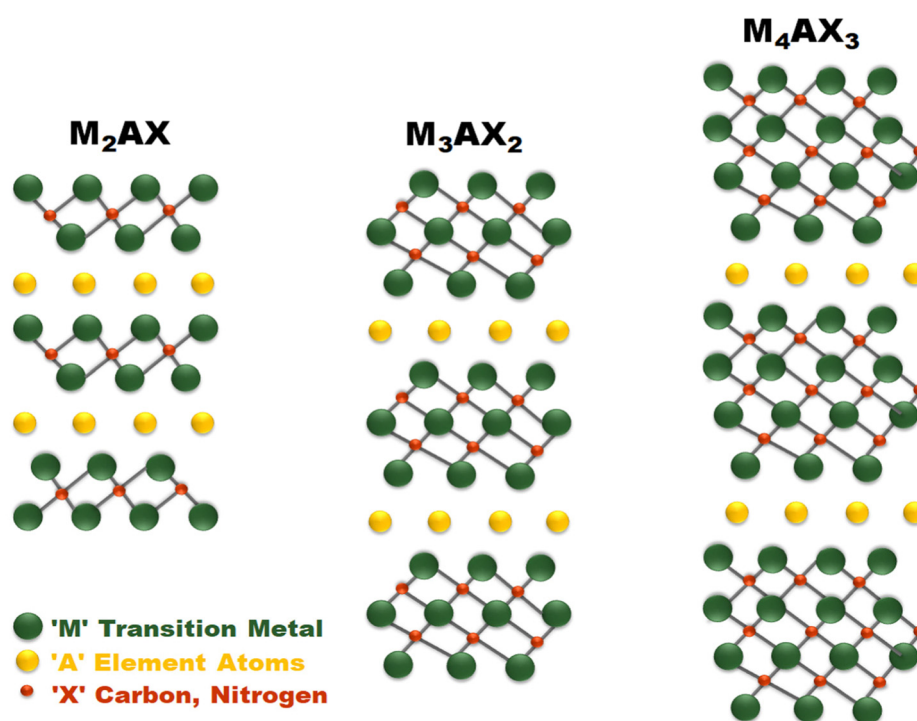
Fig. 3 MXene precursors: crystal structure of M_2AX , M_3AX_2 , and M_4AX_3 phases.
