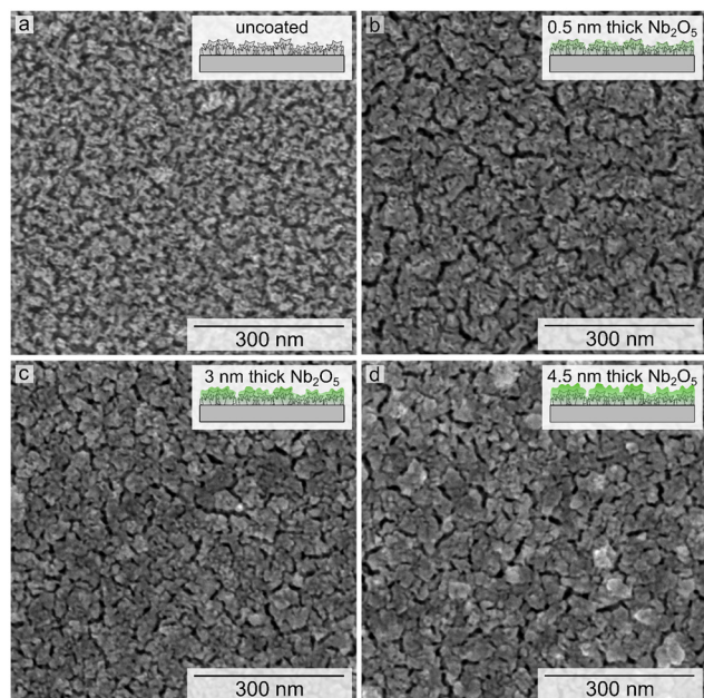
Fig. 5 A series of scanning electron microscopy (SEM) images of (a) pristine Pt with a nanoscale texture and the same substrate after coating with (b) 0.5 nm, (c) 3 nm, and (d) 4.5 nm thick layer of Nb 2 O 5 . These images were taken after 1000 cycles of an AST.
