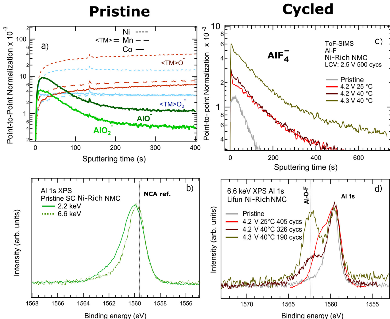
Fig. 7 a) ToF-SIMS on pristine SC Al-surface-doped-Ni-rich cathode. \langle \text{TM} \rangle = Ni, Mn, or Co, distinguished by different dashes. b) Al 1s orbital from HAXPES experiments at two different photon energies with NCA reference for \text{Al}^{3+} . 17 c) ToF-SIMS on discharged cycled Al-surface-doped-Ni-rich NMC cathode after 500 cycles to investigate the Al-F reaction product from the Al scavenger surface effect. d) HAXPES at 6.6 keV on discharged electrodes of the SC Al-surface-doped-Ni-rich material showing fluorination of Al also an indicative of Al scavenger protection from electrolyte HF attack.
