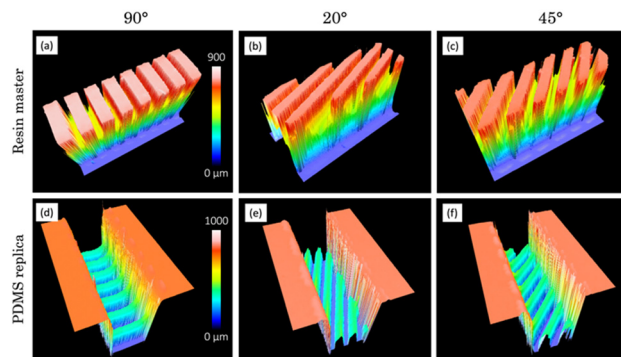
Fig. 6 3D confocal view of the micropatterned structures on the top of printed microchannels (a–c) and their corresponding PDMS replicas featuring: a) and d) 90^\circ , b) and e) 20^\circ and c) and f) 45^\circ oriented grooves.
