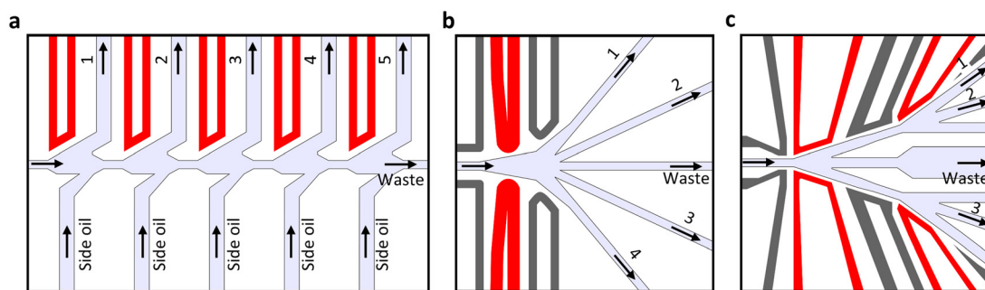
Fig. 1 Different design strategies for multiplex FADS. The microfluidic channels are represented in light-grey, the working electrodes in red and the ground electrodes in dark-grey. The different sorting outlets used in the respective studies are indicated with numbers. (a) A serial sorting design, adapted from Vyawahare et al. , 43 that consists of consecutive 2-way junctions. (b) The design principle of a parallel droplet sorting platform, consisting of one sorting junction splitting into five channels adapted from Caen et al. 6 (c) The design of the SeParate platform presented in this work, consisting of serialized 3-way junctions.
