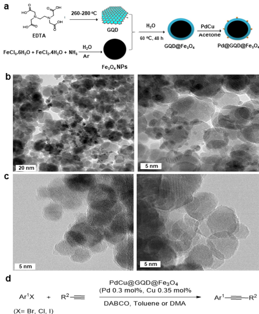
Fig. 12 (a) Schematic representation for synthesis of \text{PdCu@GQD@Fe}_3\text{O}_4 nanocatalyst; (b) TEM images \text{PdCu@GQD@Fe}_3\text{O}_4 ; (c) TEM images of \text{GQD@Fe}_3\text{O}_4 NPs and (d) Application of Sonogashira–Hagihara reaction over the catalyst \text{PdCu@GQD@Fe}_3\text{O}_4 . Reproduced with permission from ref. 151 Copyright 2017, Wiley-VCH GmbH & Co. KGaA, Weinheim.
