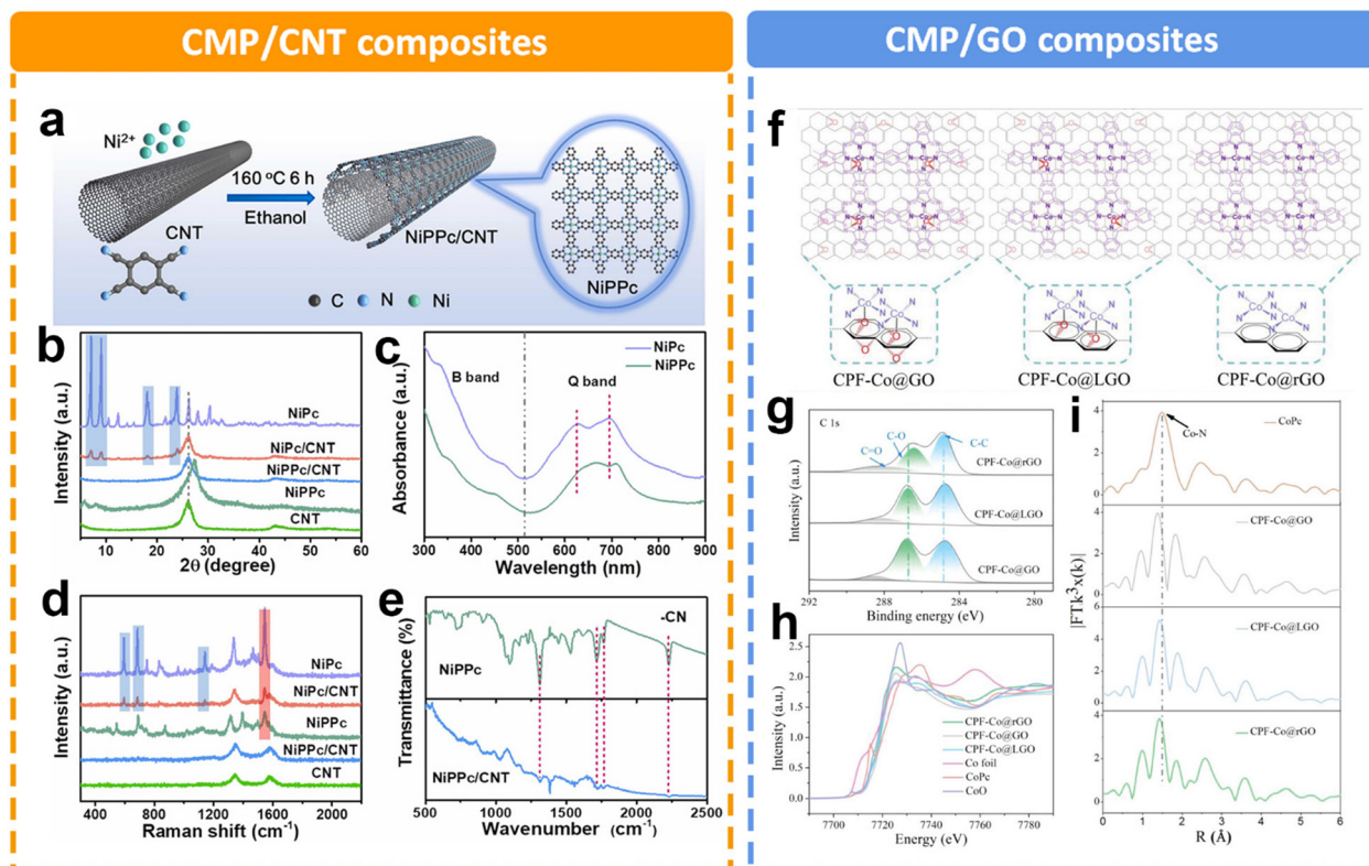
Fig. 13 Schematic illustration of different CMP composites and their characterization. (a) Schematic illustration of synthesizing NiPPc/CNTs, (b) XRD patterns of samples, (c) UV-Vis spectra of NiPPc and NiPPc in DMF, (d) Raman spectra of samples, and (e) FTIR spectra of NiPPc and NiPPc/CNT. 146 (f) Schematic illustration of the CPF-Co@GO/LGO/rGO hybrid preparation and application to electrocatalytic CO 2 to CO conversion. Structural characterization of CPF-Co@GO, CPF-Co@LGO, and CPF-Co@rGO, (g) the high-resolution C 1s XPS spectra, (h) Co K edge XANES spectra, and (i) Co K-edge FT of the EXAFS spectra. 147
