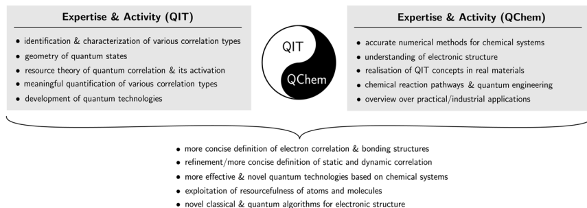
Fig. 1 Illustration of the expertise and activities within quantum information theory (QIT) and quantum chemistry (QChem), and anticipated potential synergy with and emphasis on the electron correlation problem and the ongoing second quantum revolution (see text for more details).
