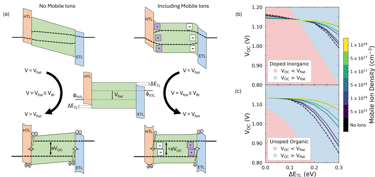
Fig. 1 (a) Illustration of the impact of mobile ions on solar cell band diagrams. In these figures, we assume undoped organic transport layers. \Delta E_{TL} is defined as the energetic offset between the perovskite's conduction (valence) band and that of the ETL (HTL). The built-in potential ( V_{BI} ) is defined as the difference in the equilibrium values of the anode and cathode work function ( \phi_{HTL} and \phi_{ETL} , respectively). In the central panel, where the applied voltage is equal to the flat band condition in the active layer, V_{flat} , the band diagrams of devices with and without mobile ions look identical. Note how, in this example, the residual band bending in the undoped contacts means that V_{flat} < V_{BI} . In the bottom row, we illustrate how band bending due to the redistribution of mobile ions can reduce minority carrier accumulation at interfaces, when compared to an equivalent device with no ions. This reduces the rate of interfacial recombination for a given applied voltage, increasing the device's open circuit voltage ( V_{OC} ). Figures (b) and (c) show the dependence of V_{OC} on \Delta E_{TL} for doped inorganic and undoped organic parameter sets, respectively. The red and blue shaded regions indicate where V_{OC} is less than and greater than V_{flat} , respectively.
