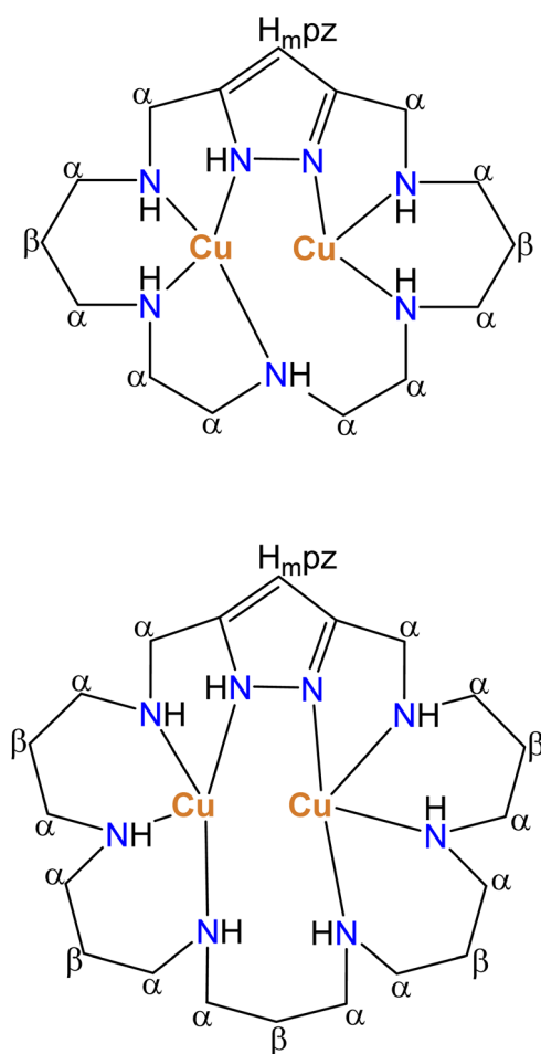
Scheme 2 Nitrogen coordination pattern found in binuclear \text{Cu}^{2+} complexes of L1 and L3 suggested by paramagnetic ^1\text{H} NMR spectra.
