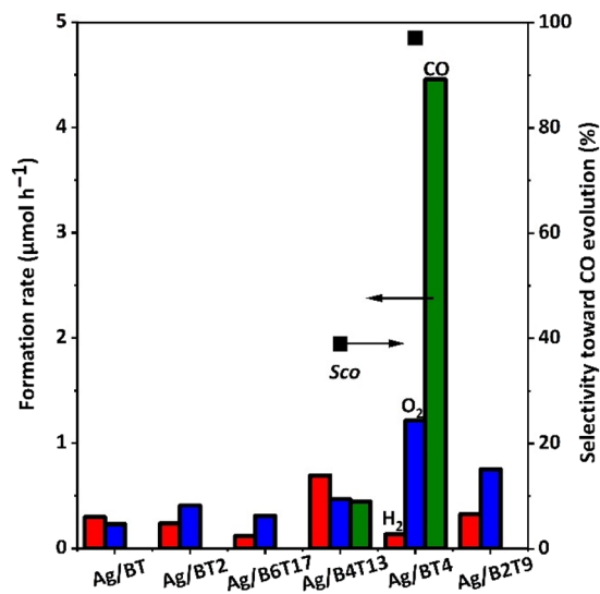
Fig. 2 Formation rates of \text{H}_2 (red), \text{O}_2 (blue), and \text{CO} (green), and selectivity for \text{CO} evolution ( S_{\text{CO}} , square) in the photocatalytic reaction test for \text{CO}_2 reduction with water under photoirradiation over the barium titanate samples with 1 wt% Ag cocatalyst.
